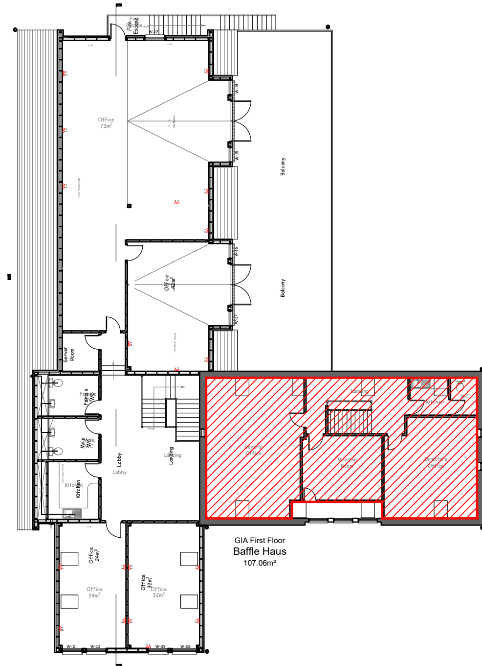
First Floor
