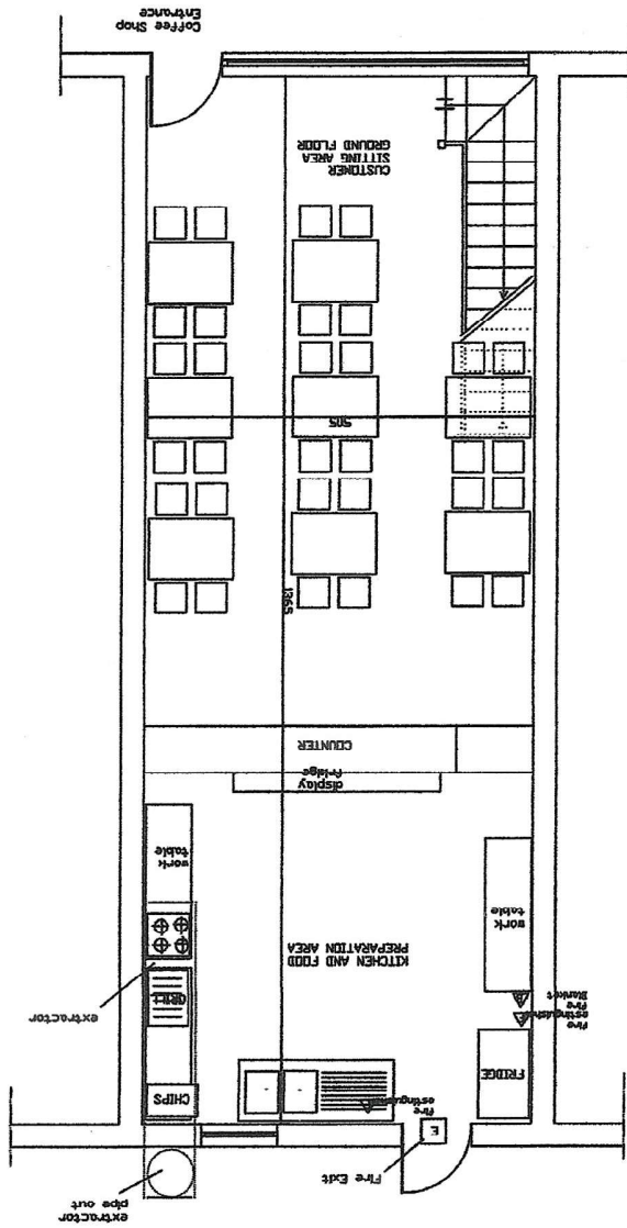
GROUND FLOOR PROPOSED PLAN COFFEE SHOP SCALE: 1/100
