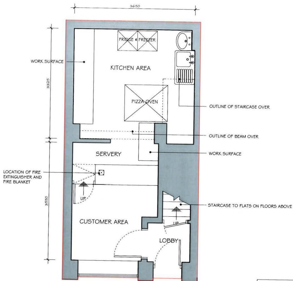
FLOOR PLAN SCALE 1:50 @ A4
